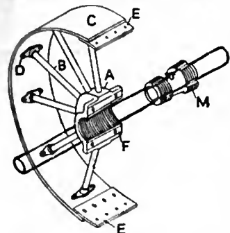
FIG. 1.—Built-up Pulley. passing through the flanges F, and the pulley is connected to the
