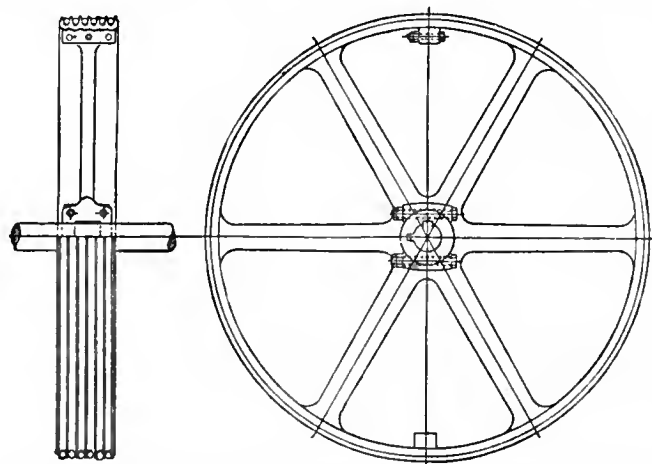
FIG. 5.—Rope Pulley, 10 ft. diam., 6 grooves, 2 1/2 in. pitch, weight about 35 cwt. Constructed by Combe, Barbour & Combe, Ltd., Belfast.
