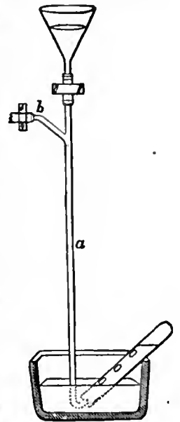
FIG. 4. Sprengel's Air-Pump.
