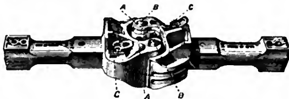
FIG. 28.—Automatic Coupling for Freight Cars (U.S.A.).
