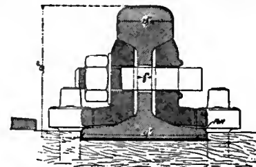
FIG. 12.—French Rail, 90½ lb to the yard, showing rail joint and seat in the sleeper.
