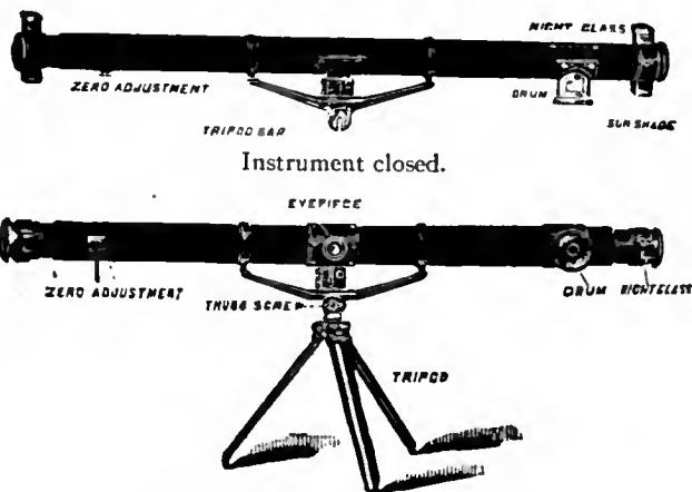
FIG. 4.—Marindin Range-Finder.
