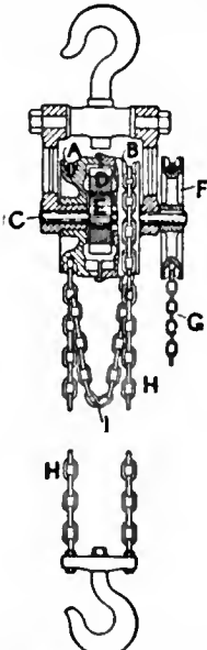
FIG. 7.—Moore and Head Pulley Block.
