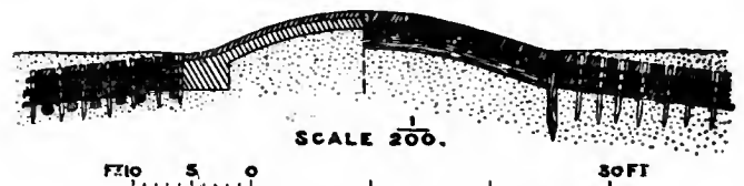
FIG. 10.—Sections of Groynes at Blankenberghe.
